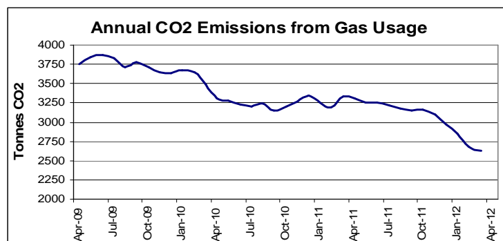
Figure 1.10: CO 2 emissions arising from gas consumption
